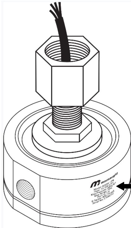
Flow Meter Details
