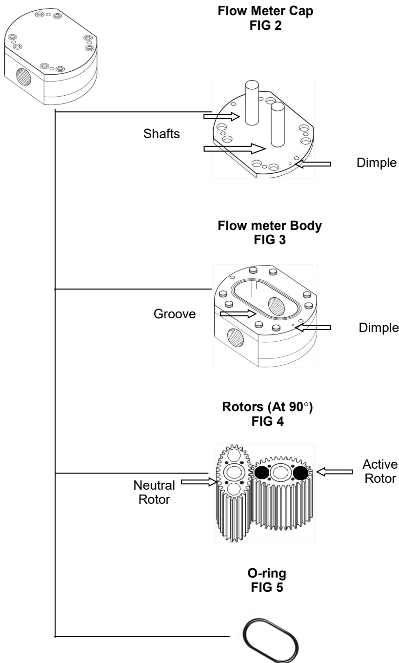
Flow meter FIG 1
