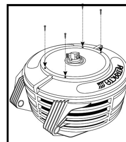
11) Fit screws.
